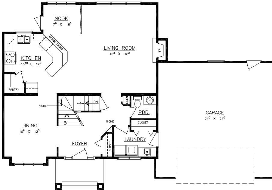
MAIN FLOOR AREA = 966 S.F.
